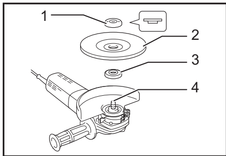
► 1. Lock nut 2. Depressed center grinding wheel/Multi-disc 3. Inner flange 4. Spindle
